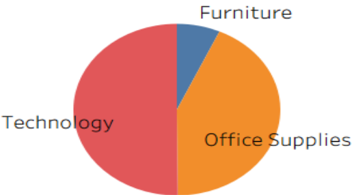
Pie chart
